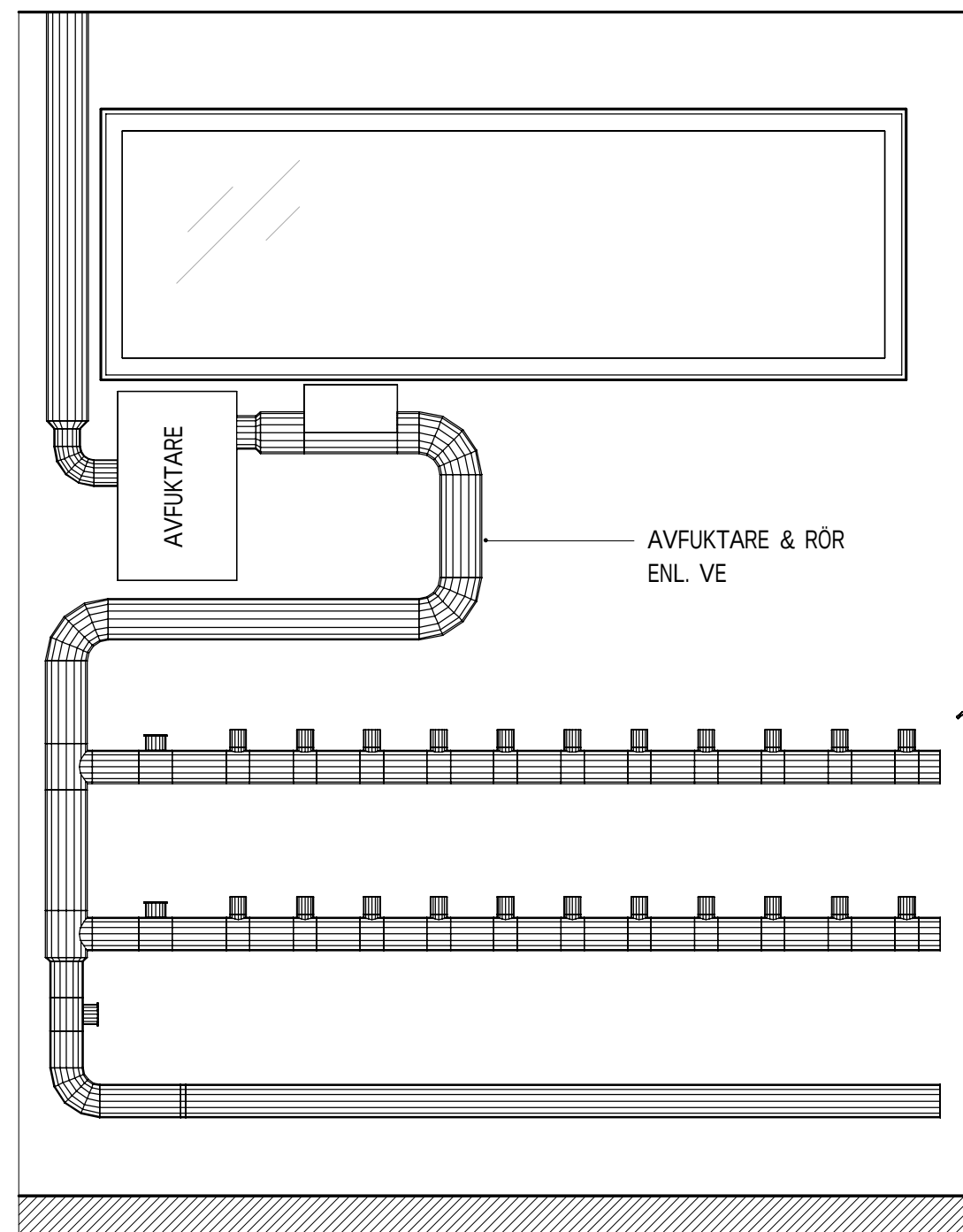
ELEVATION TORKRUM 1002 - C 1 : 20
