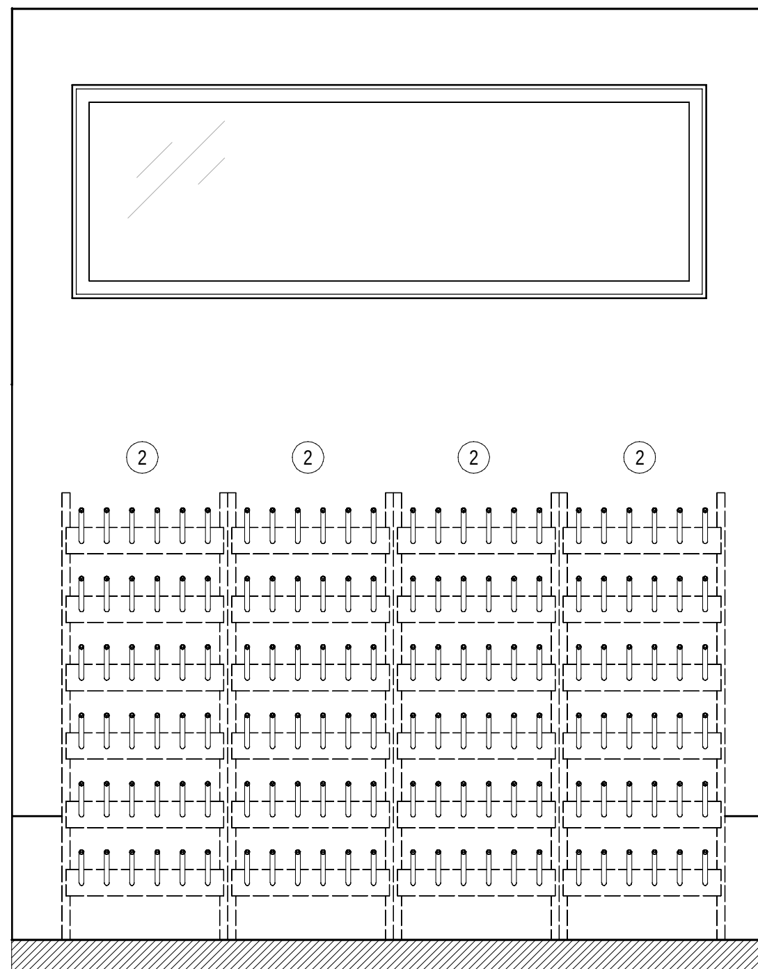
ELEVATION TOROKRUM 1002 - A 1 : 20
